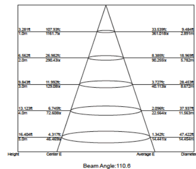
Illuminance-Distance Curve
