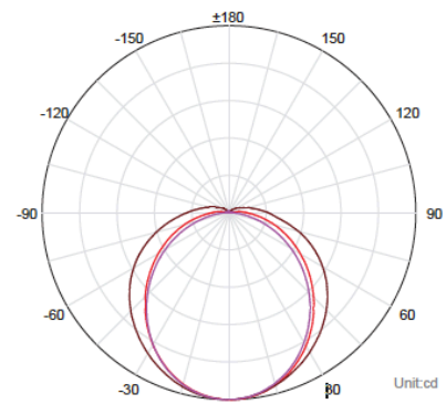
C Plane Distribution Diagram
