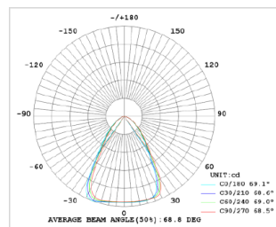
60° PC lens
