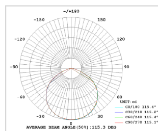
120° PC lens
