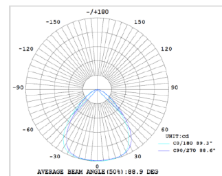
90° PC lens
